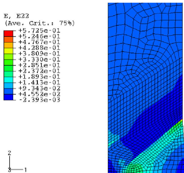
Figure A-6. Strain Distribution in Butt Weld with Lower Strength (including 70% hoop stress/yield stress)
