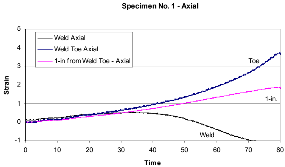
Figure A-16. Strain Versus Time for Al Tube without Pressure
