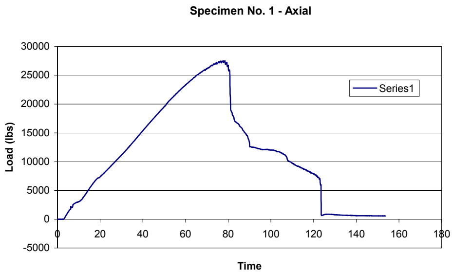
Figure A-17. Load Versus Time for Al Tube without Pressure
