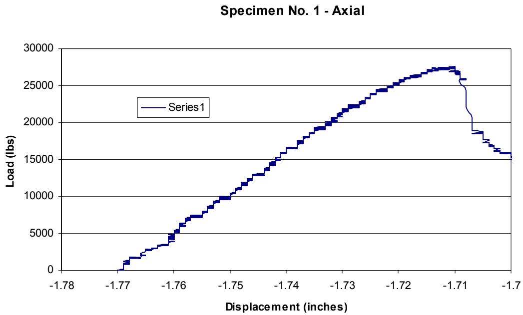
Figure A-18. Load Displacement Results for Al Tube without Pressure
