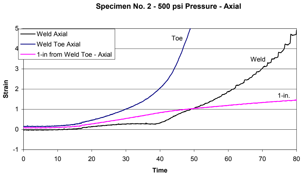
Figure A-19. Strain Versus Time for Al Tube with Internal Pressure
