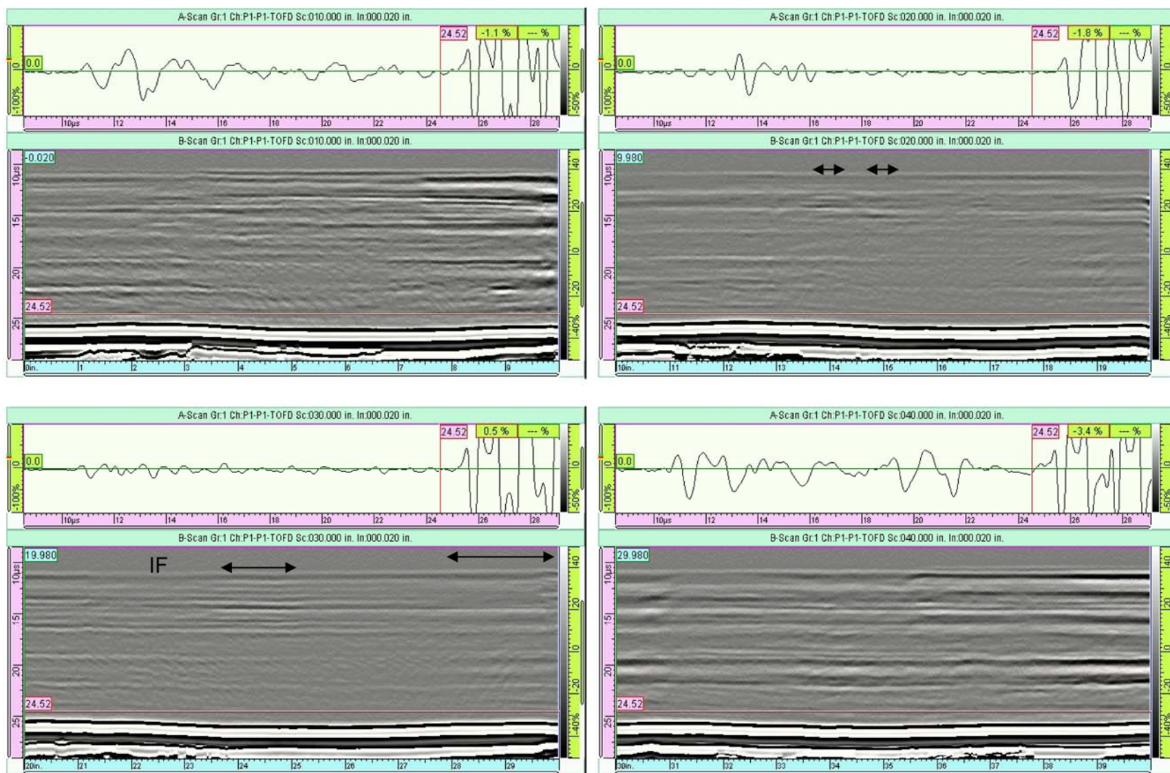
Figure B.2. HDPE Pipe 122, Condition 1
