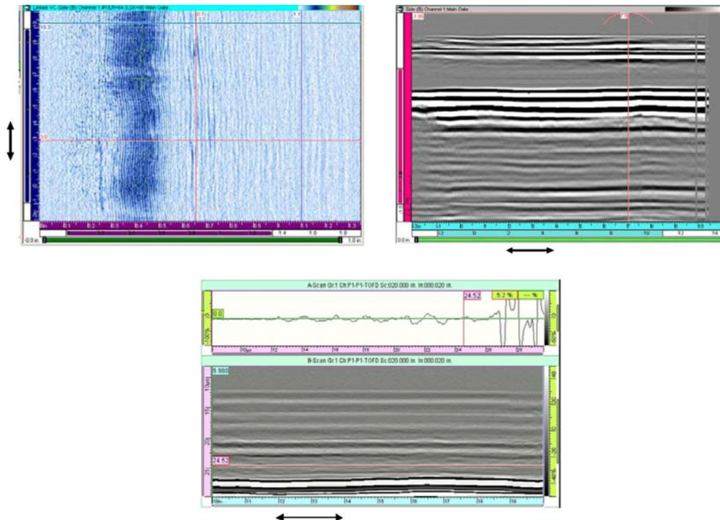
Figure 4.9. Ultrasonic Responses from Quadrant Two of Pipe 1224 All Show No Flaw Indication. The PNNL PA data is in the upper left, PNNL TOFD data in the upper right, and Fluor/NDT Innovations, Inc. TOFD data in the bottom.
