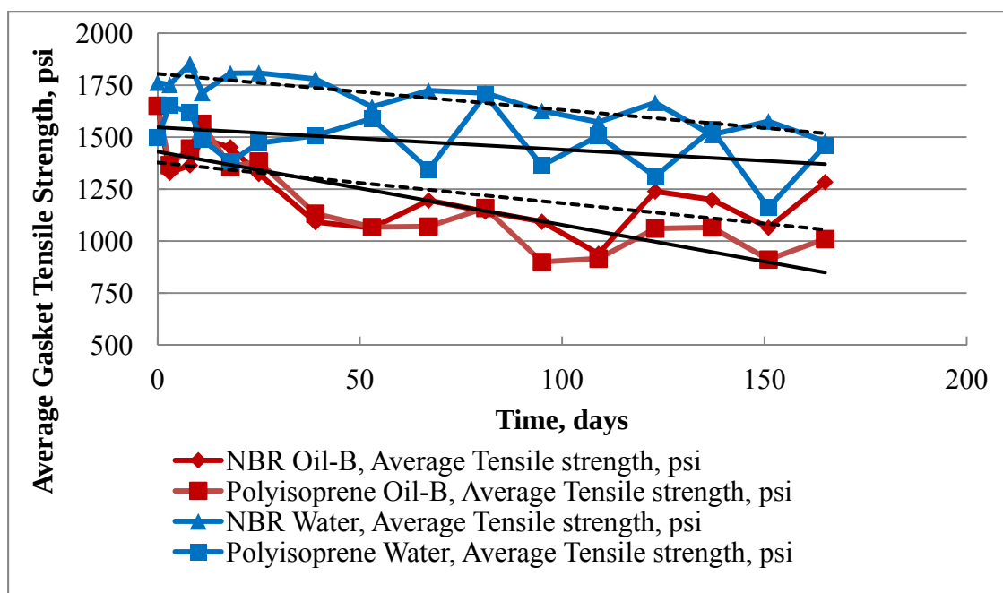
Figure 4.11. Average tensile strength of gaskets submerged in water and Oil-B.
